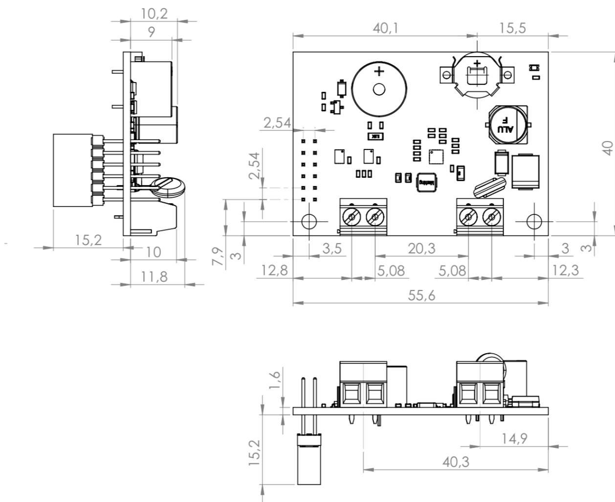
DIMENSIONS (mm)
